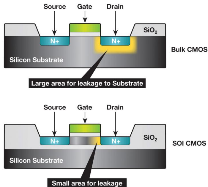
Figure 4: Comparison of leakage-current paths of bulk CMOS and SOI CMOS.
