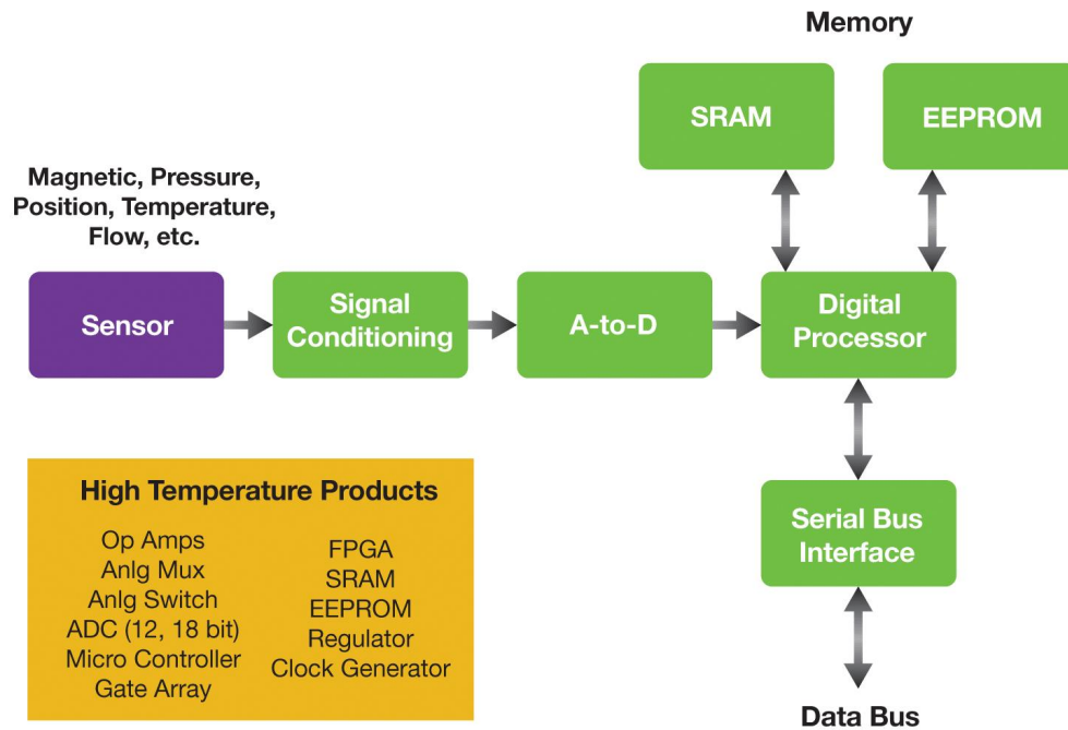
Figure 6: Data acquisition block diagram
