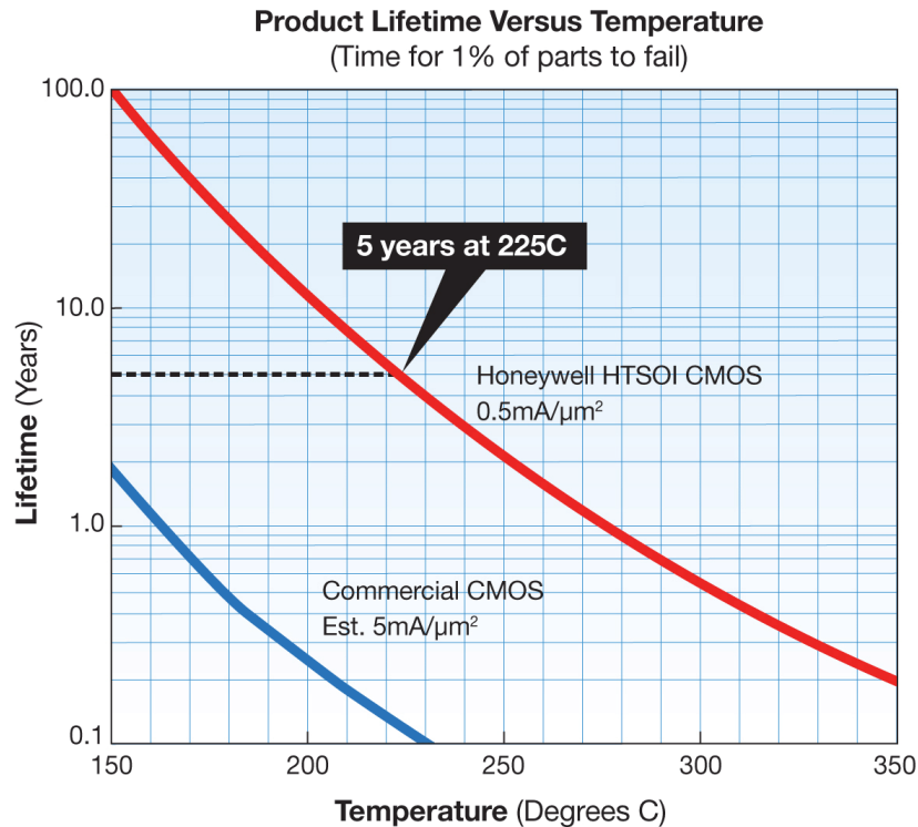
Figure 7: Semiconductor lifetime based on electromigration
