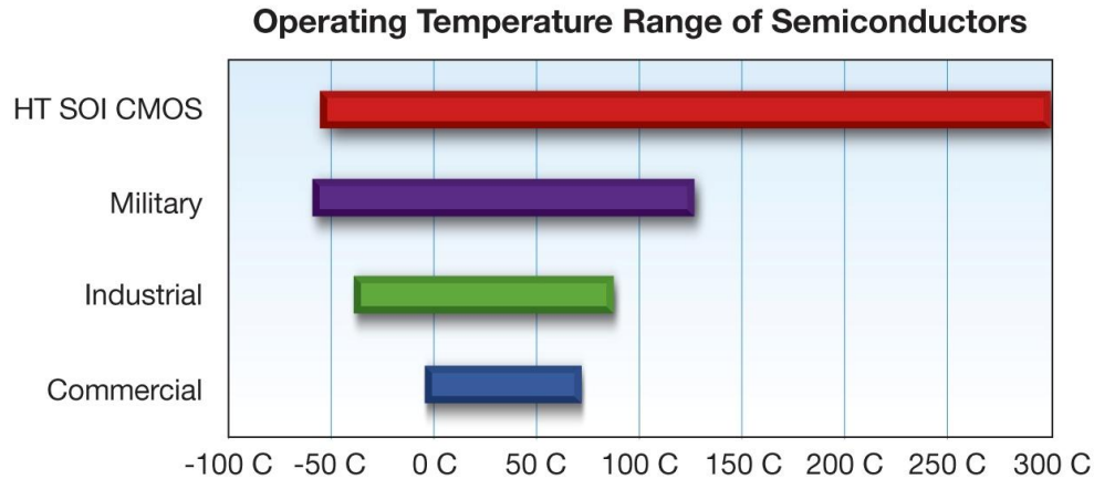
Figure 2: Semiconductor temperature ranges
