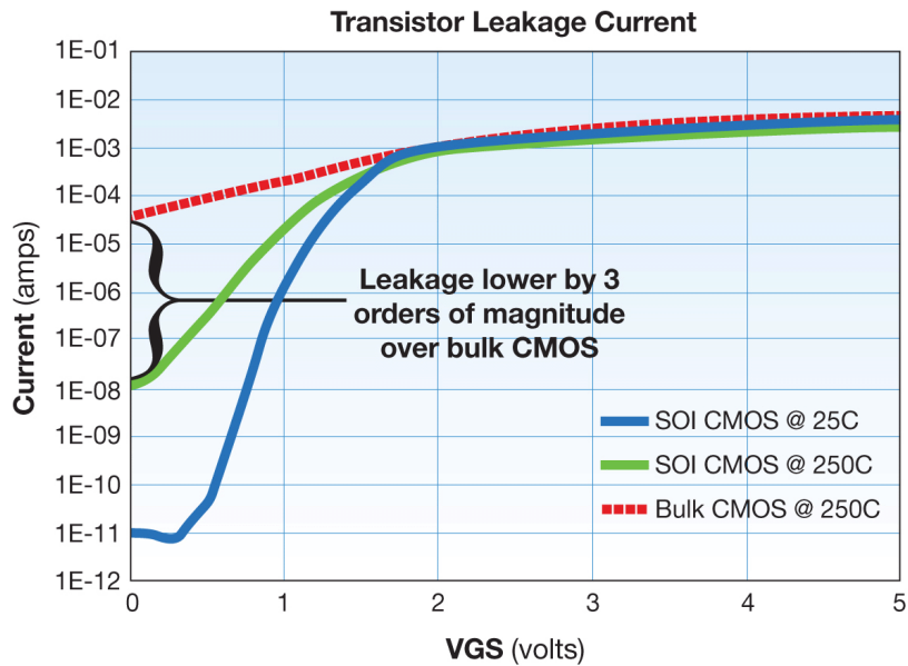
Figure 5: Comparison of transistor leakage current between SOI CMOS and bulk CMOS
